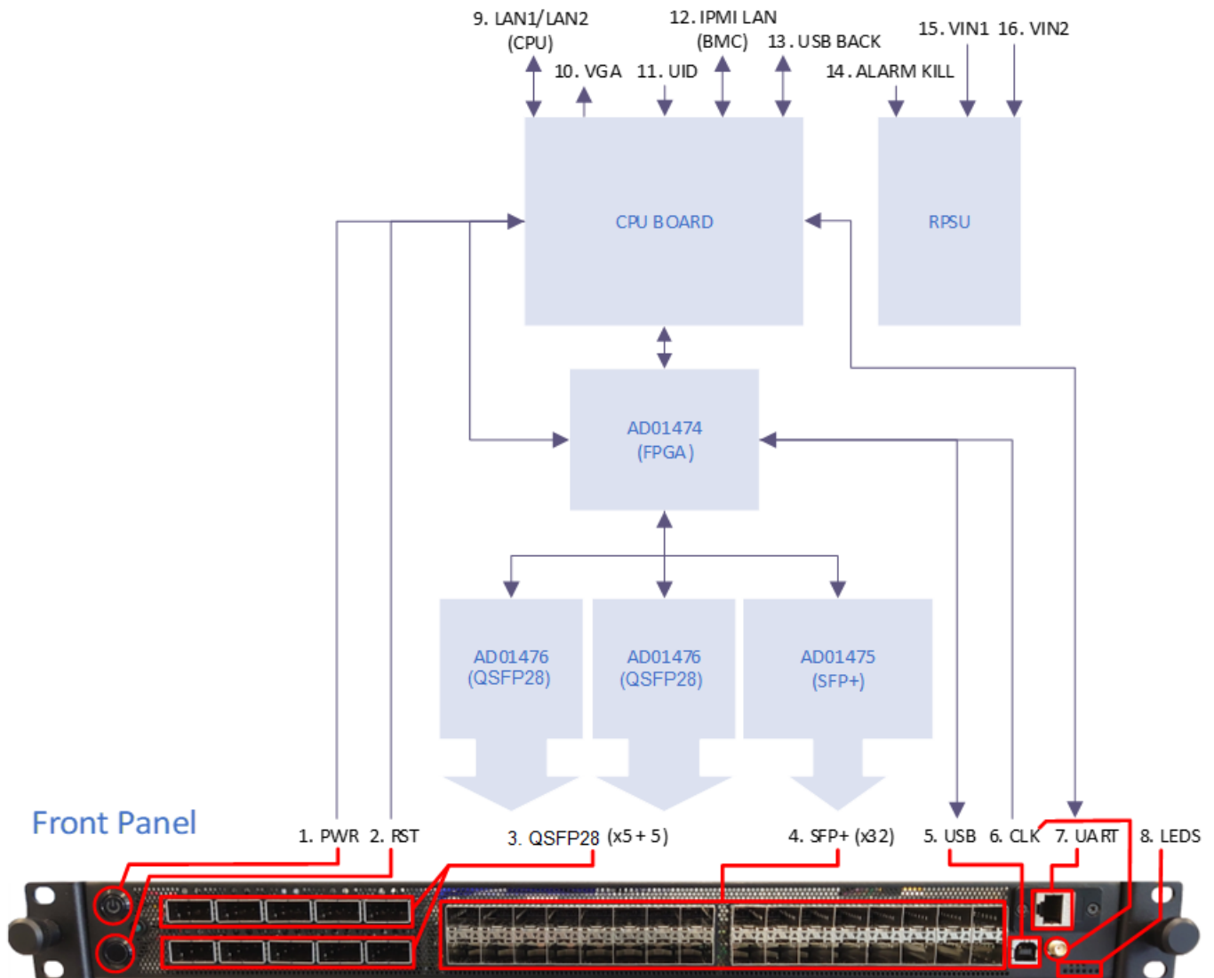
Figure 4 : Interfaces
