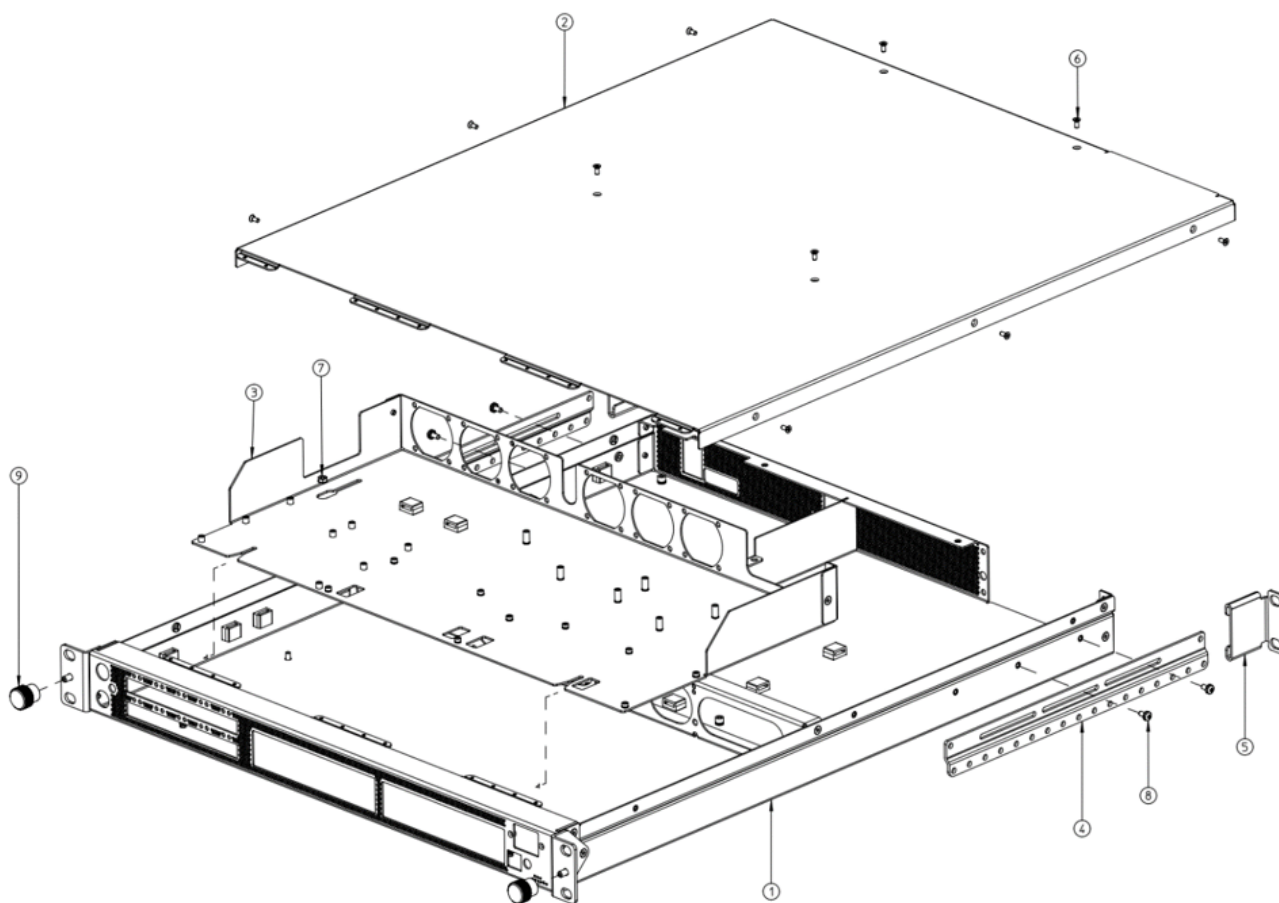
Figure 5 : Chassis Elements
