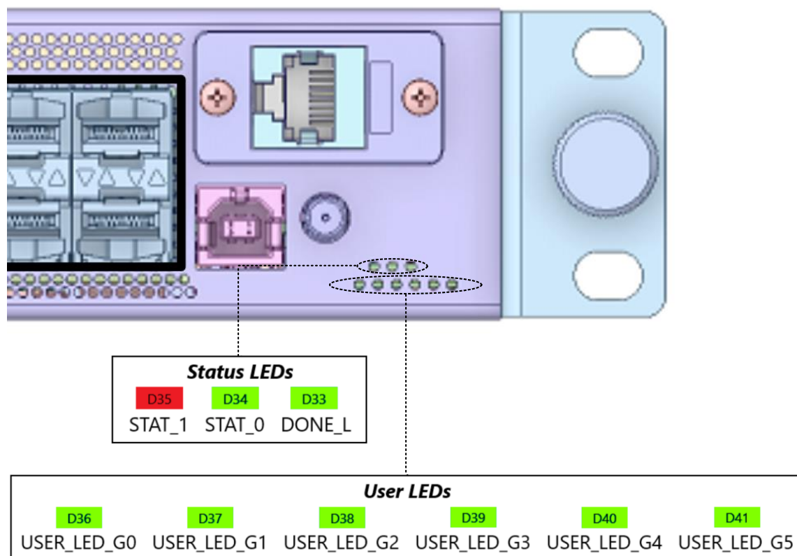
Figure 9 : Front Panel LEDs
