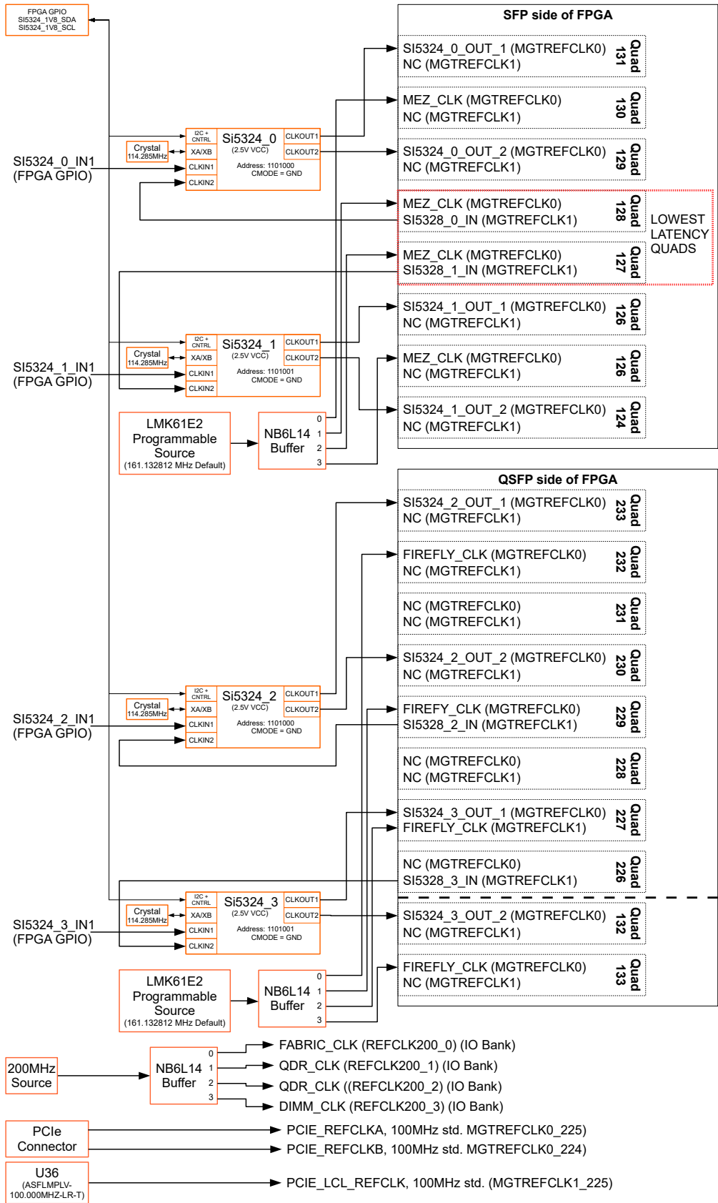
Figure 13 : Clock Topology
