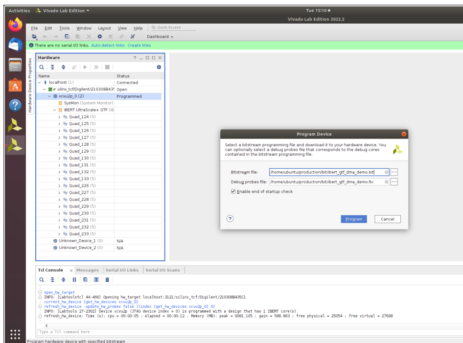
Figure 19 : Reprogramming the FPGA
