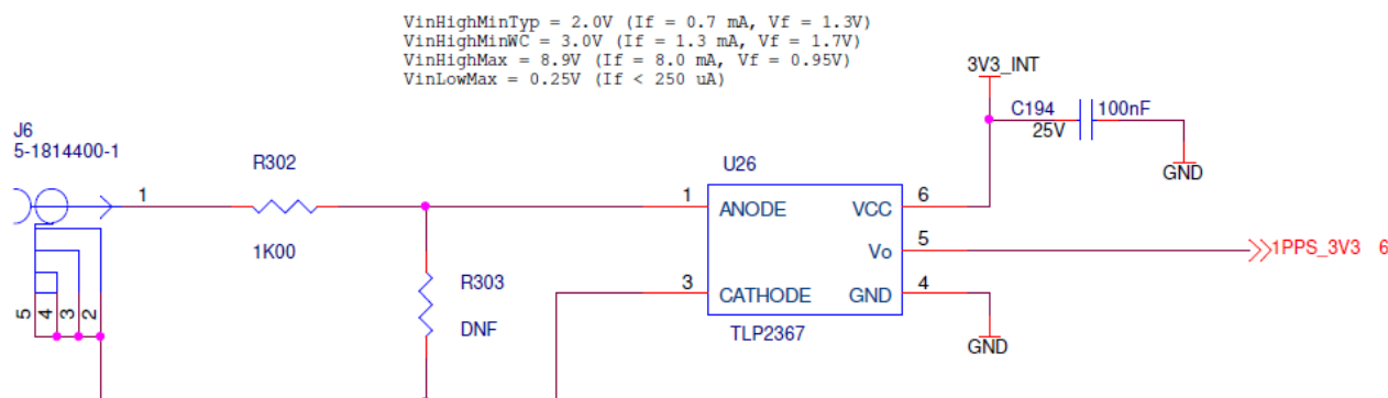
Figure 8 : 1PPS circuit
