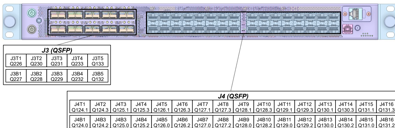
Figure 12 : Front Panel QSFP/SFP connections to the AD01474
