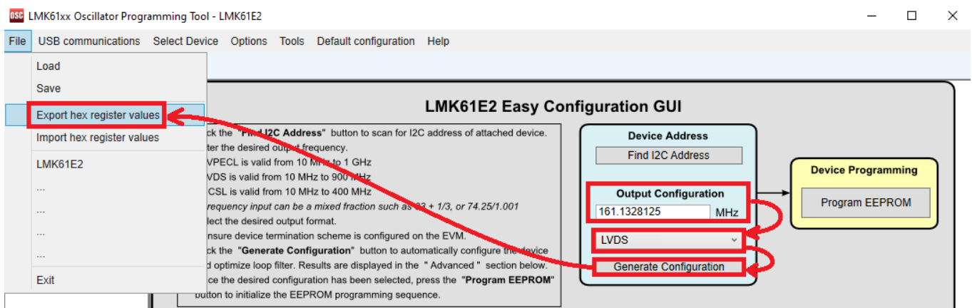
Figure 14 : LMK61xx Oscillator Programming Tool GUI
