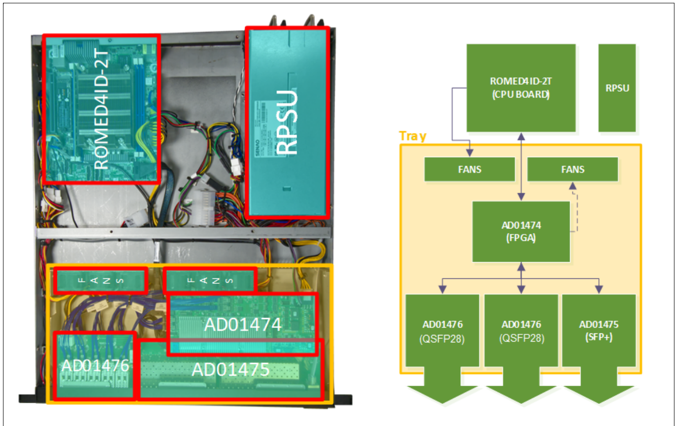
Figure 3 : ADA-R9100 HW modules
