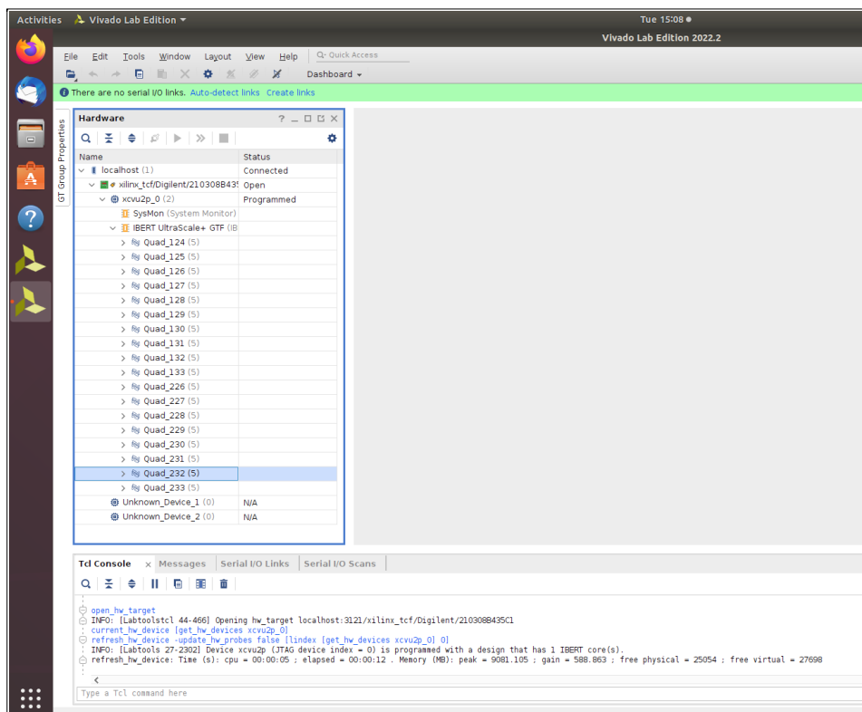
Figure 18 : Scanning the JTAG chain for the FPGA
