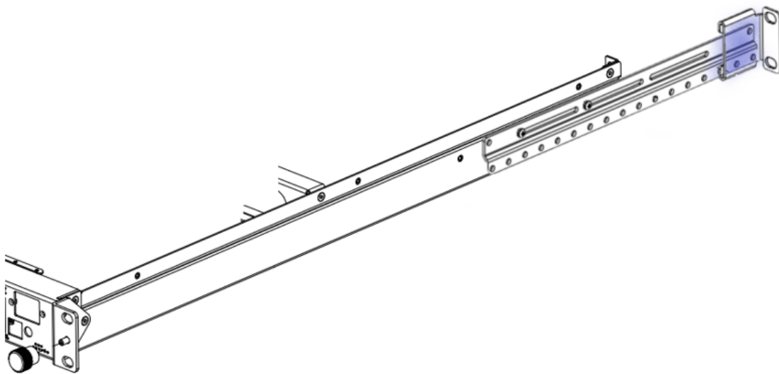
Figure 7 : Adjusting the rails extension to the rack depth
