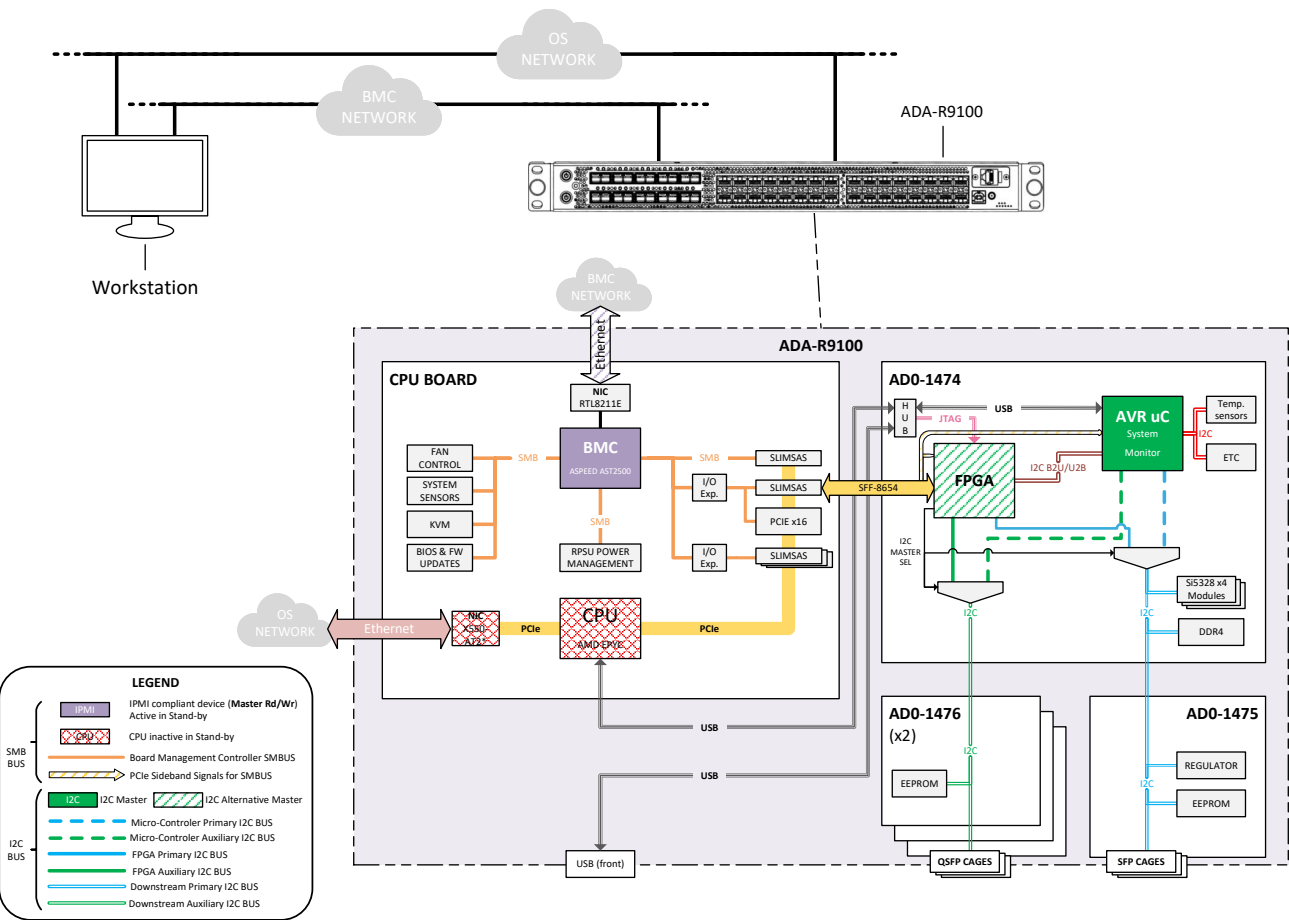
Figure 31 : ADA-R9100 IPMI And I2C Architecture
